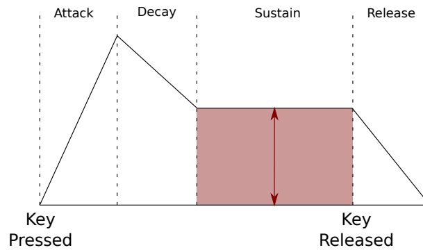
Figure 286: Sustain on ADSR Envelope
